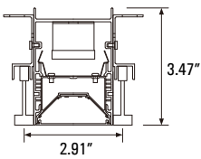
9/16" Slot-1
