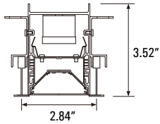
9/16" Flat
