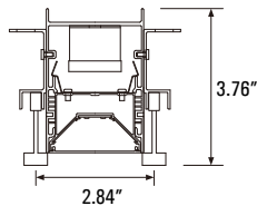
9/16" Slot-2
